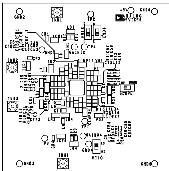
Figure 114. AD8334-EVALZ Assembly
