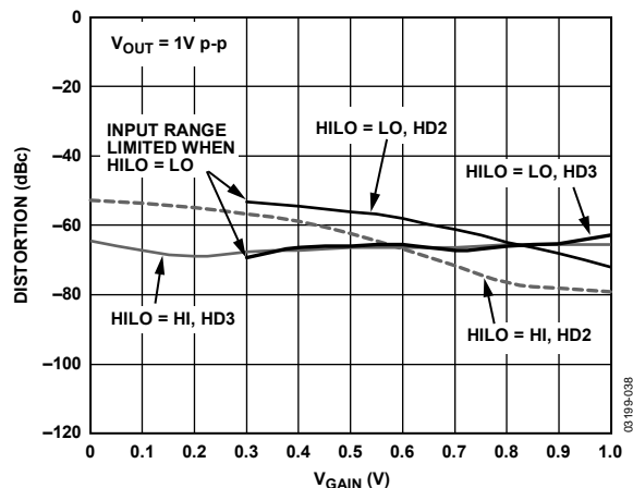
Figure 38. Harmonic Distortion vs. V_{GAIN} , f = 10\text{ MHz}
