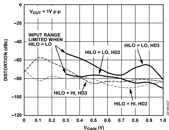
Figure 37. Harmonic Distortion vs. V_{GAIN} , f = 1\text{ MHz}
