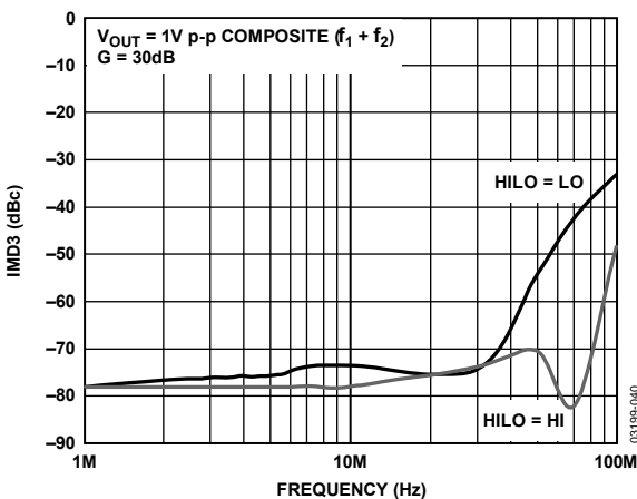
Figure 40. IMD3 vs. Frequency
