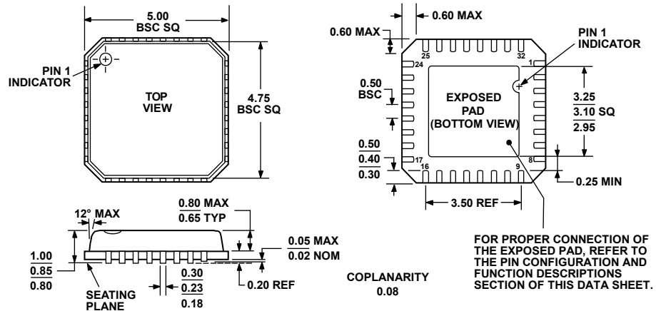
Figure 124. 32-Lead Lead Frame Chip Scale Package (LFCSP_VQ)
