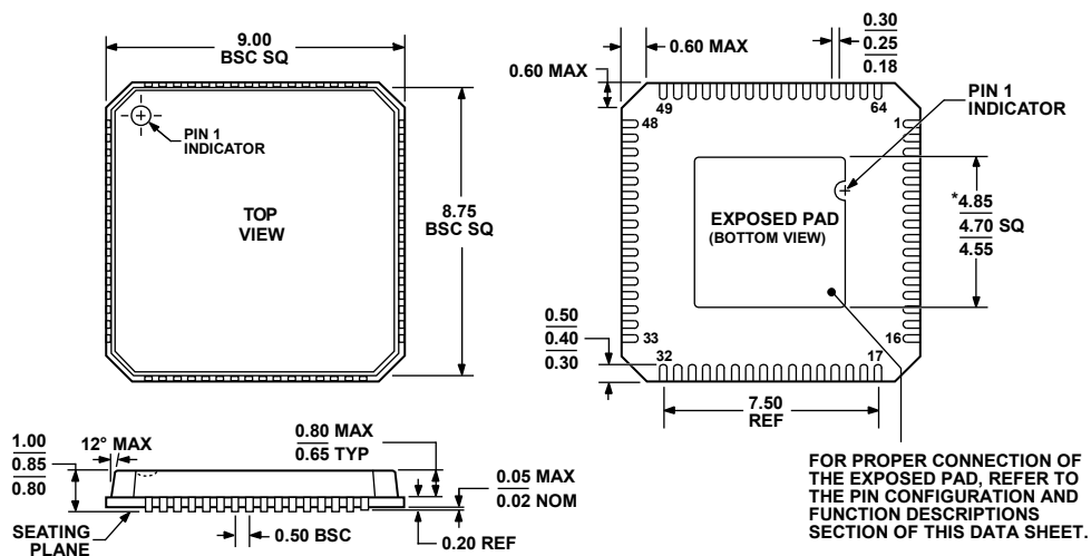
Figure 125. 64-Lead Lead Frame Chip Scale Package (LFCSP_VQ)
