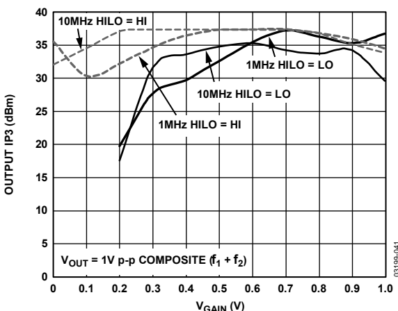
Figure 41. Output Third-Order Intercept (IP3) vs. V_{GAIN}
