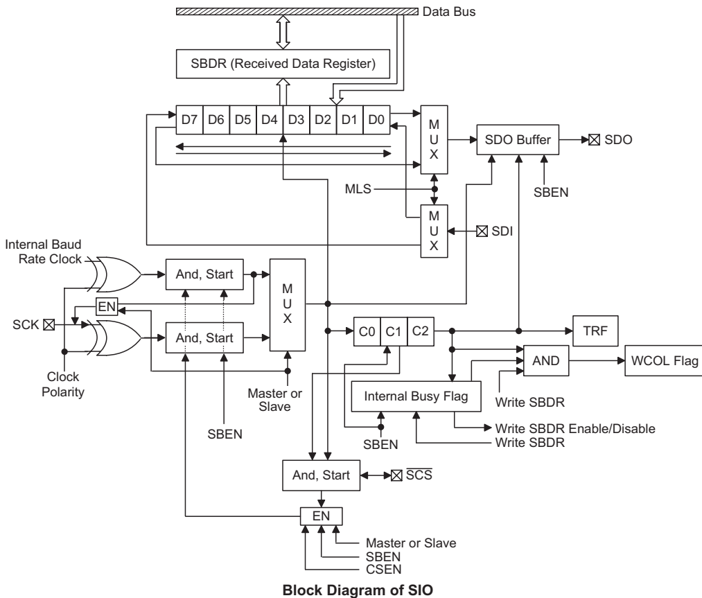
Block Diagram of SIO
