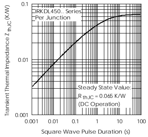
Fig. 13 - Thermal Impedance Z_{thJC} Characteristic
