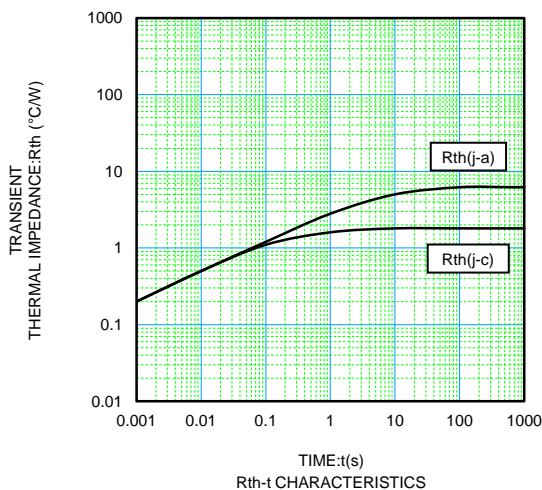
TIME:t(s) Rth-t CHARACTERISTICS
