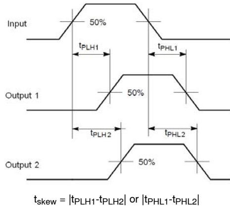
Figure 13. Bit-to-Bit and Channel-to-Channel Skew
