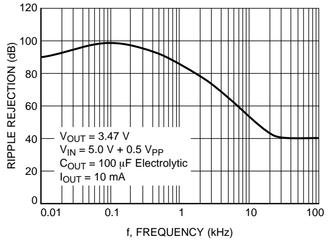
Figure 10. Ripple Rejection
