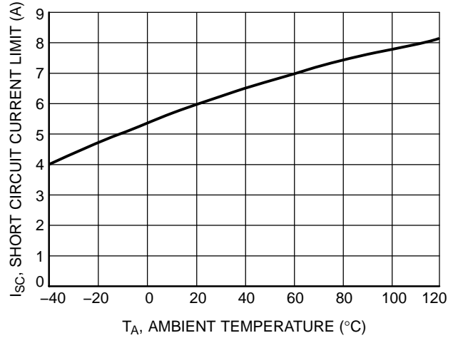
Figure 4. Short Circuit Current Limit versus Temperature
