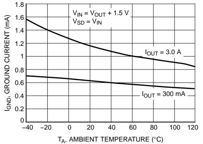
Figure 6. Ground Current versus Temperature
