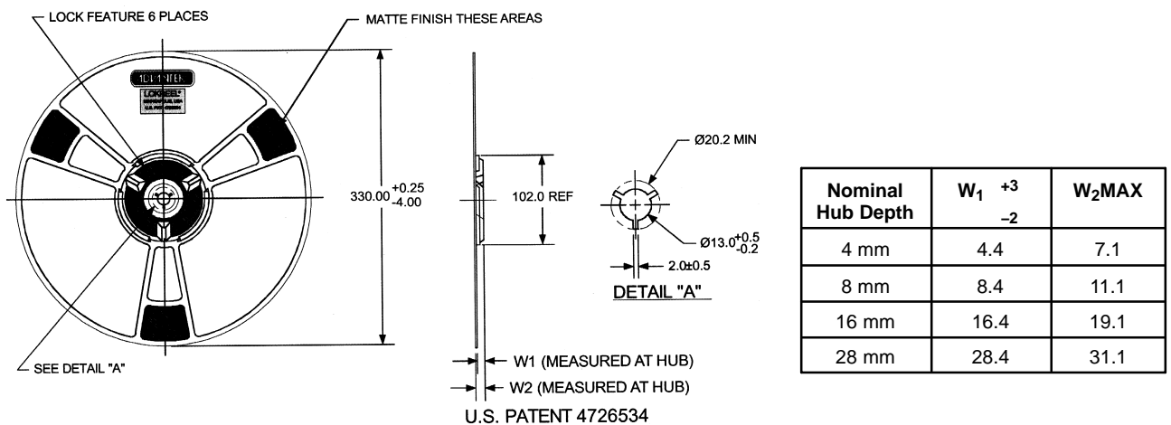
Figure 13. Reel Dimensions
