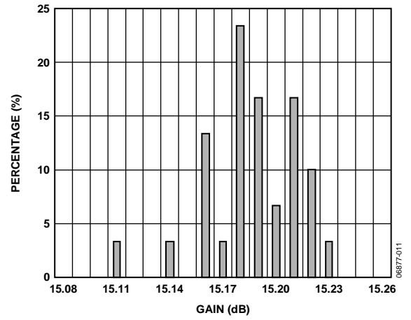
Figure 11. Gain Distribution at 900 MHz
