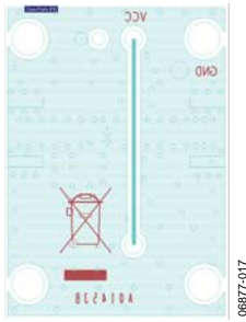
Figure 17. Evaluation Board Layout (Bottom)
