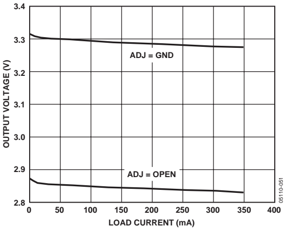
Figure 7. LDO Output Voltage vs. Load Current, V_{IN} = 5\text{ V}
