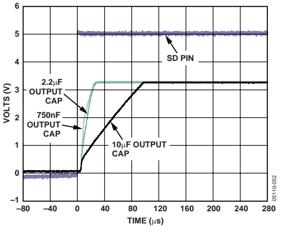
Figure 8. LDO Power-Up Response from Shutdown
