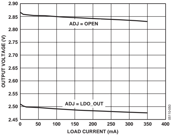
Figure 6. LDO Output Voltage vs. Load Current, V_{IN} = 3.3\text{ V}
