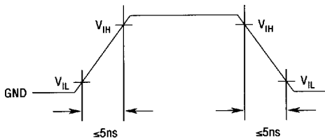
Input Waveforms
