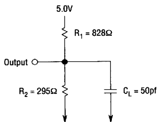
Load Circuit
