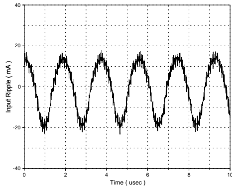
Input Ripple Current
