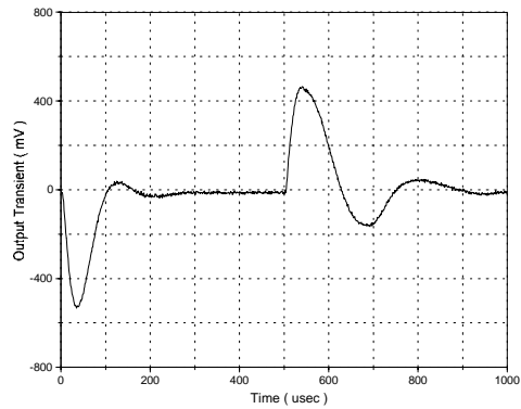
Output Load Transient Response 10% Load to/from 50% Load
