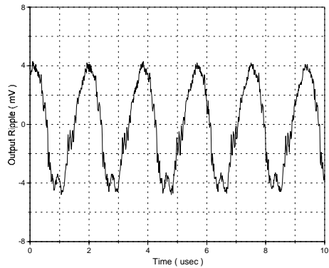
Output Ripple Voltage
