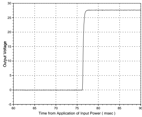
Turn-on Time, No Load
