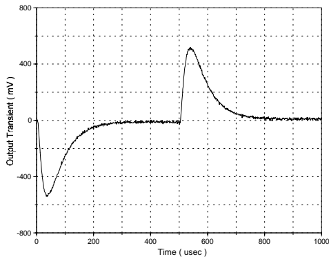
Output Load Transient Response 50% Load to/from 100% Load
