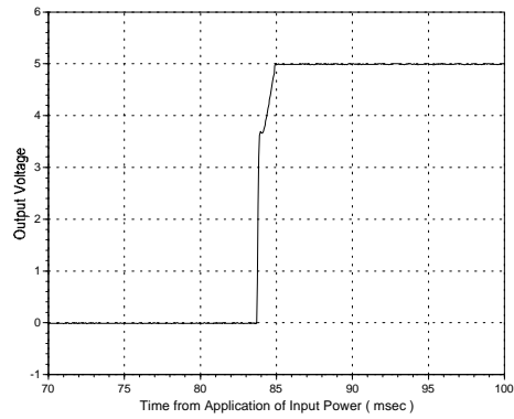
Turn-on Time, Full Load
