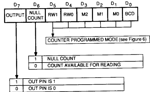
Figure 11 : STATUS BYTE
