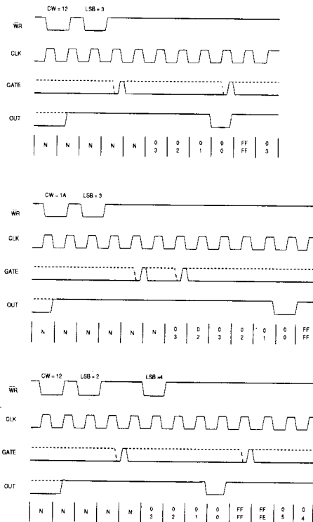
Figure 18 : MODE 5 TIMING
