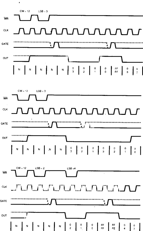
Figure 14 : MODE 1 TIMING
