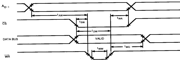
Figure 4 : TIMING DIAGRAMS
