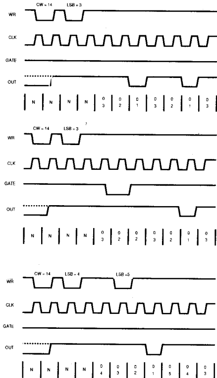
Figure 15 : MODE 2 TIMING
