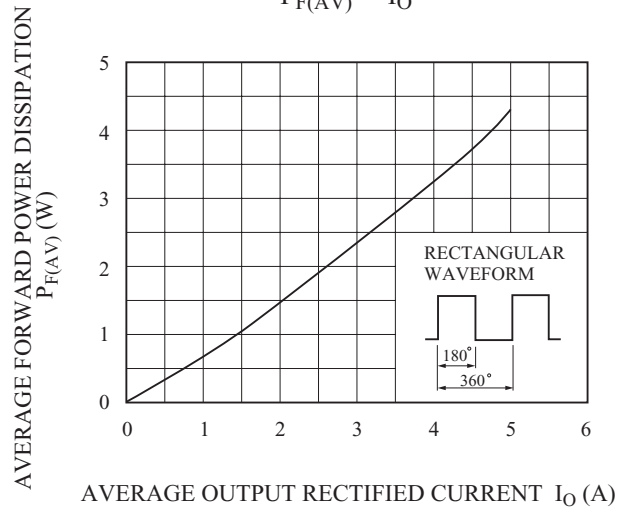
P_{F(AV)} - I_O
