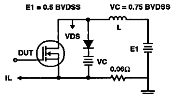
FIGURE 2. CLAMPED INDUCTIVE SWITCHING, ILM
