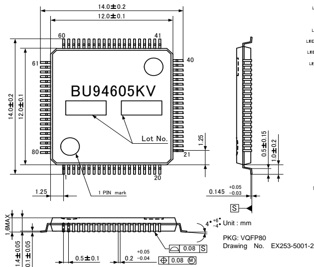
Figure 1. External dimension
