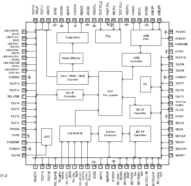
Figure 2. Block diagram
