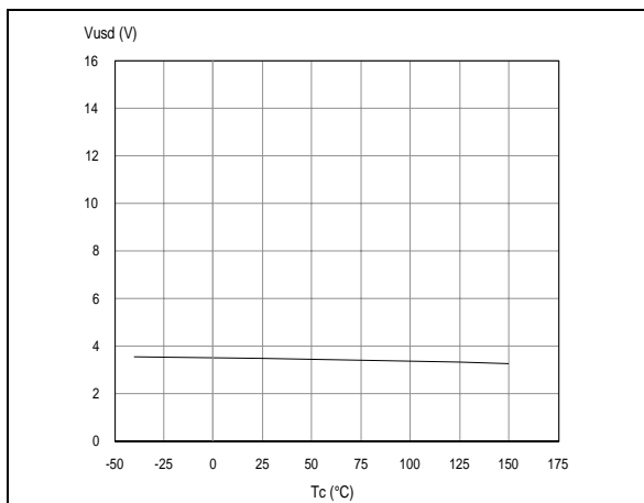
Figure 14. Undervoltage shutdown
