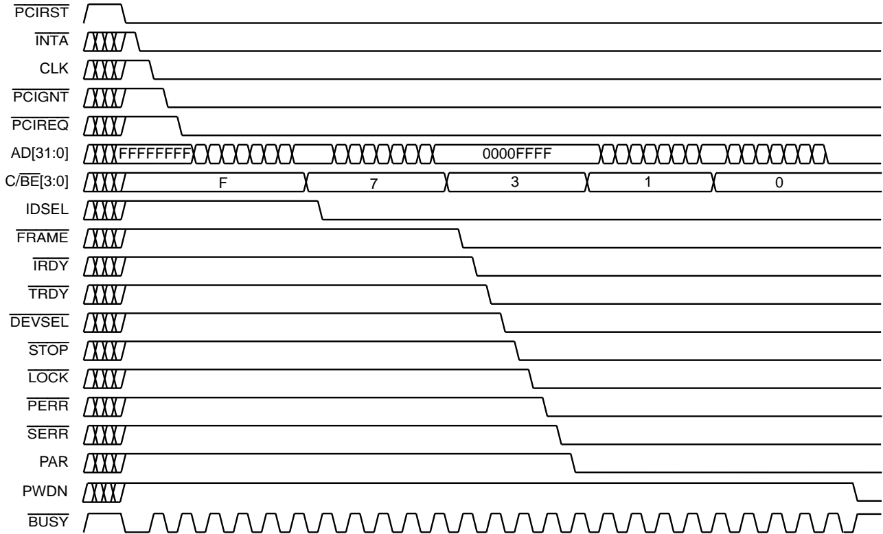
Figure 2-3 NAND Tree Waveform
