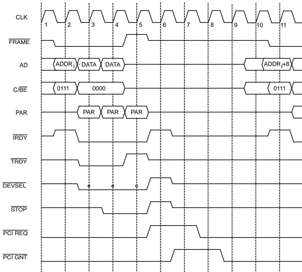
Figure 4-10 Disconnect With Data Transfer
