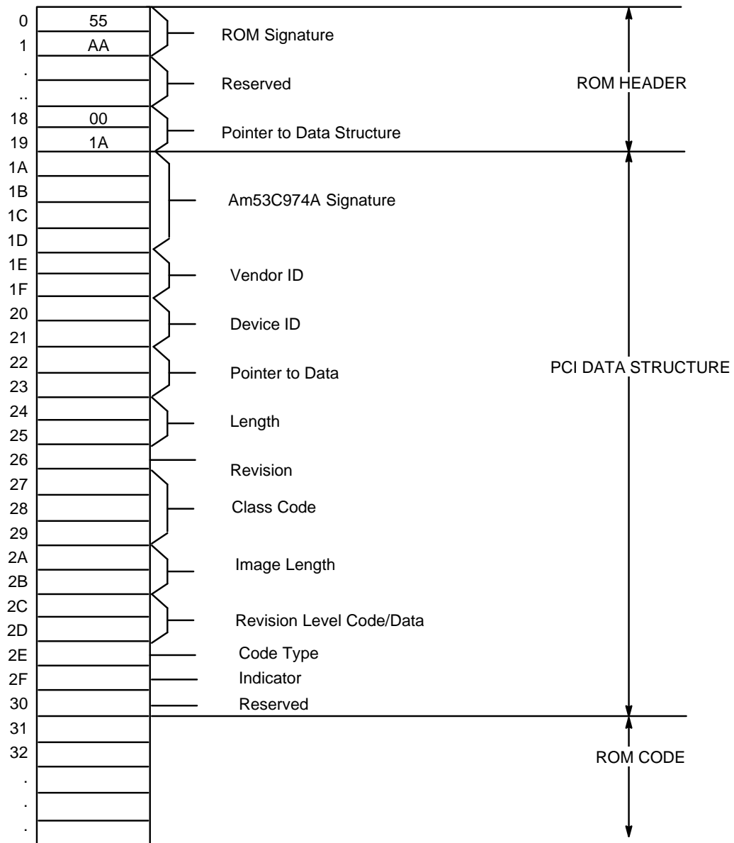
Figure 7-5 Am53C974A Expansion ROM Mapping
