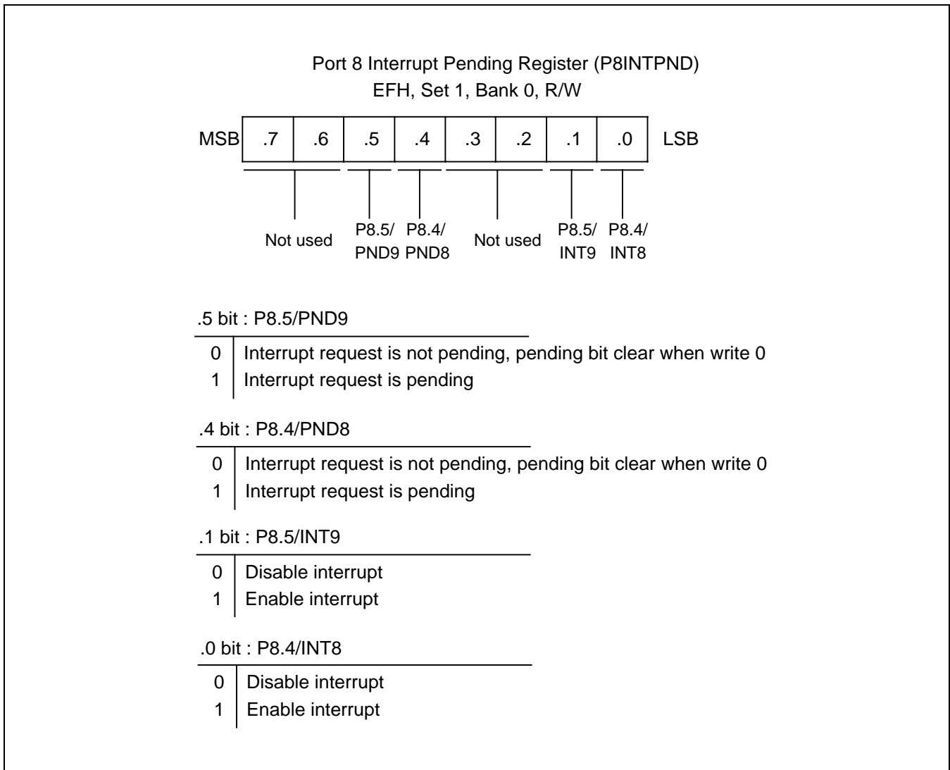
Figure 9-16. Port 8 Interrupt Pending Register (P8INTPND)
