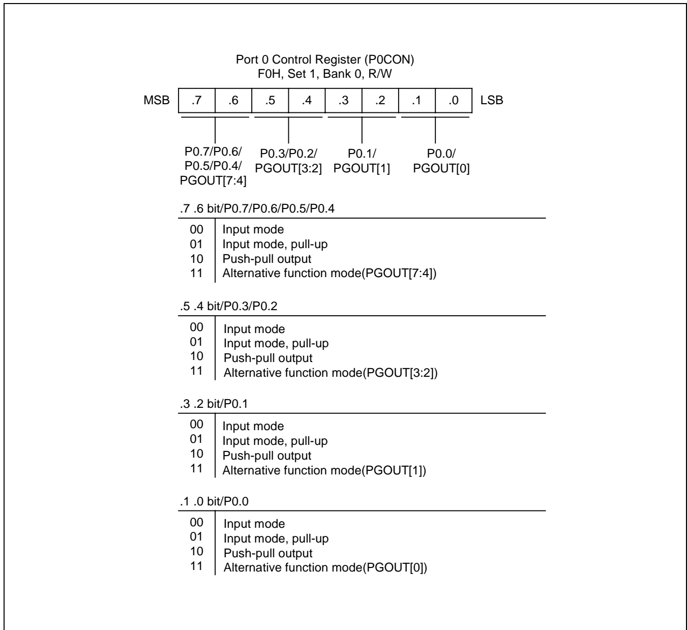
Figure 9-1. Port 0 Control Register (P0CON)
