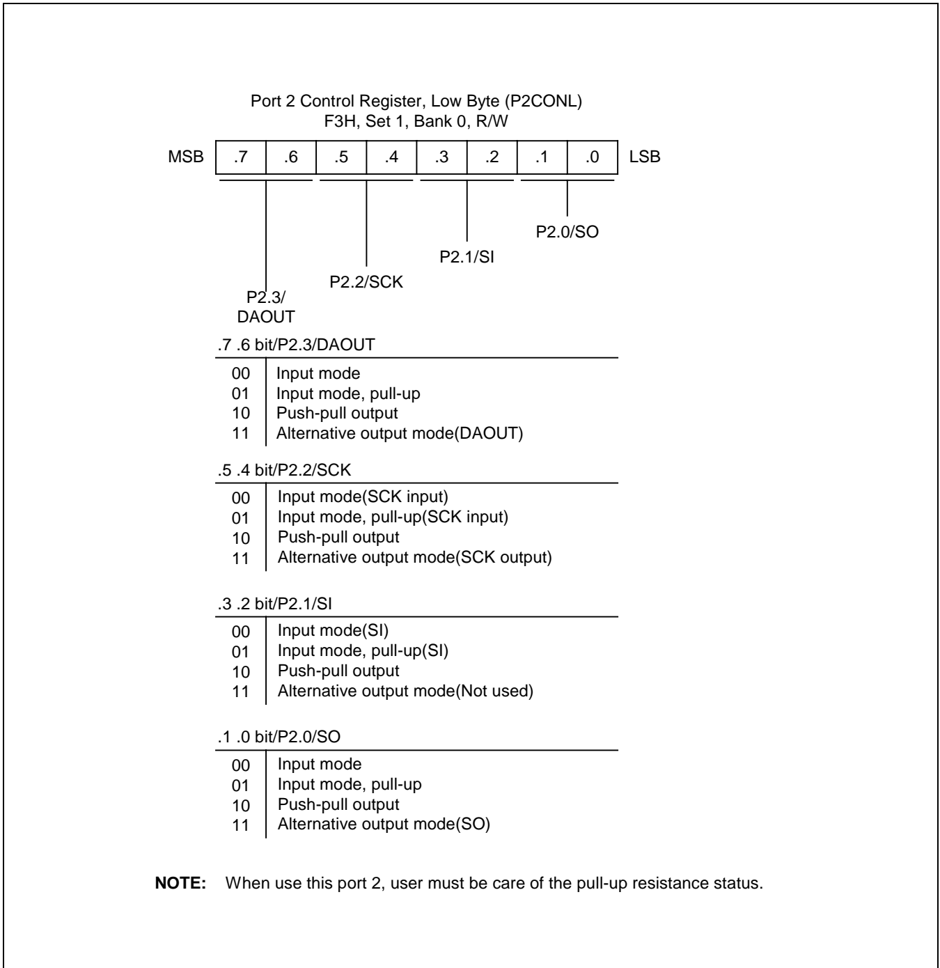
Figure 9-4. Port 2 Low-Byte Control Register (P2CONL)
