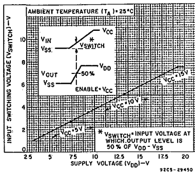
Fig. 9 - Typical input switching as a function of high-level supply voltage. (SELECT at V CC -CMOS mode).
