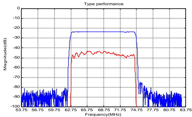
SP68B11 SAW Filter Typical Performance
