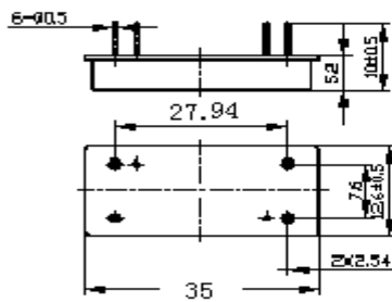
Package Outline
