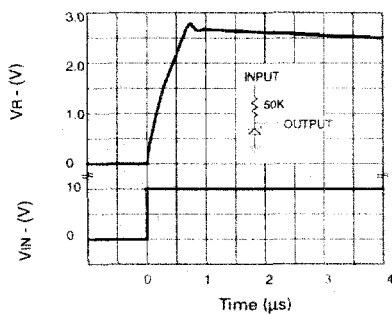
Transient Response (IR=150µA)
