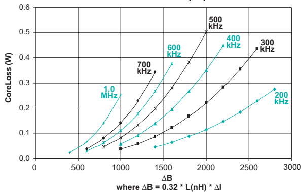
CoreLoss (W)
