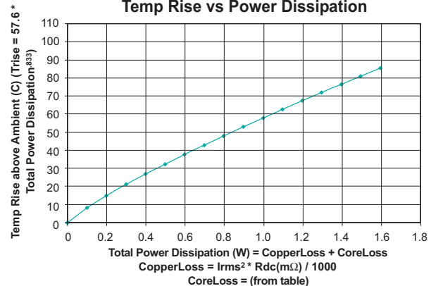
Temp Rise vs Power Dissipation
