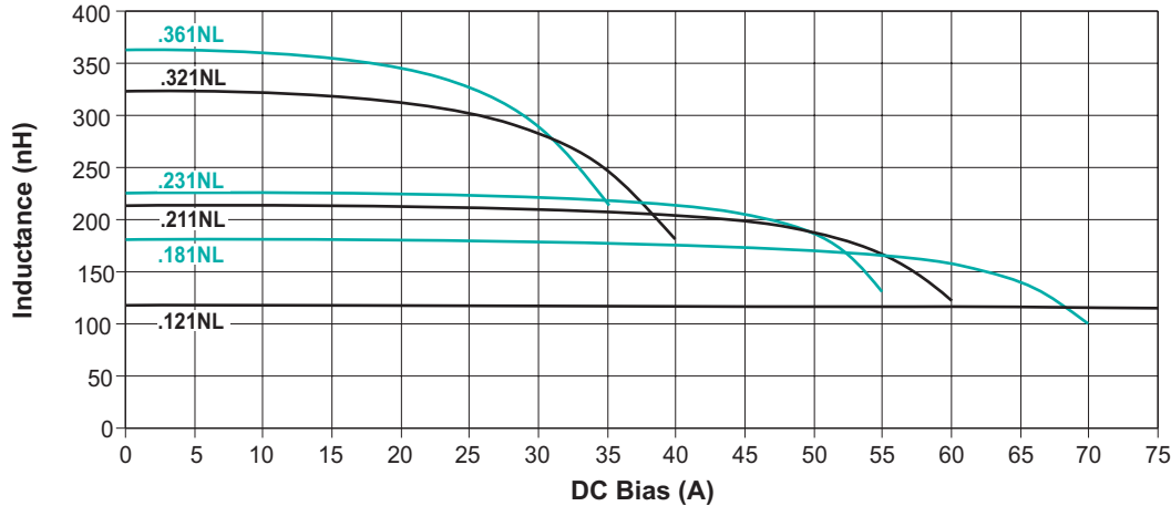
Typical Inducance vs DC Bias @ 100°C
