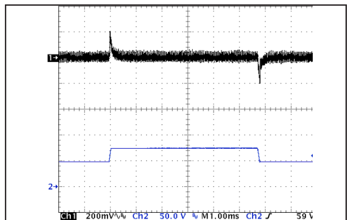
Figure 6: Output voltage response to step-change in input voltage (nominal to maximum, 1000 V/ms). Load cap: 15 \mu F tantalum and 1 \mu F ceramic capacitors. Ch 1: Vout, Ch 2: Vin.
