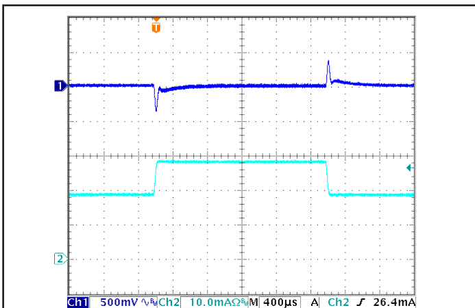
Figure 5: Output voltage response to step-change in load current (66%-100%-66% of Iout(max)); di/dt = 0.1 \text{ A}/\mu\text{s} . Load cap: 15µF tantalum and 1µF ceramic capacitors. Ch 1: Vout, Ch 2: Iout (5 A/div).
