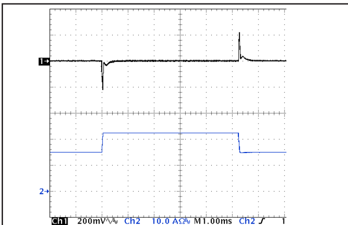
Figure 5: Output voltage response to step-change in load current (66%-100%-66% of Iout(max); di/dt = 0.1 A/\mu s ). Load cap: 15 \mu F tantalum and 1 \mu F ceramic capacitors. Ch 1: Vout, Ch 2: Iout (10 A/div).
