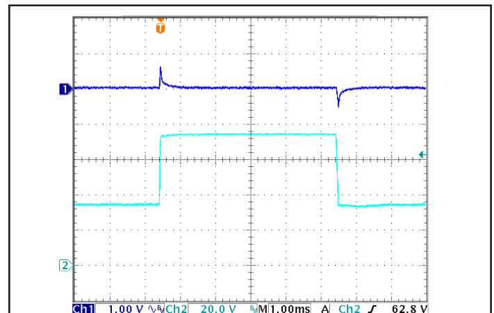
Figure 6: Output voltage response to step-change in input voltage (nominal to maximum, 1000 V/ms). Load cap: 15µF tantalum and 1µF ceramic capacitors. Ch 1: Vout, Ch 2: Vin.
