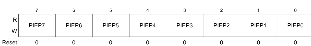
Figure 24-42. Port P Interrupt Enable Register (PIEP)
