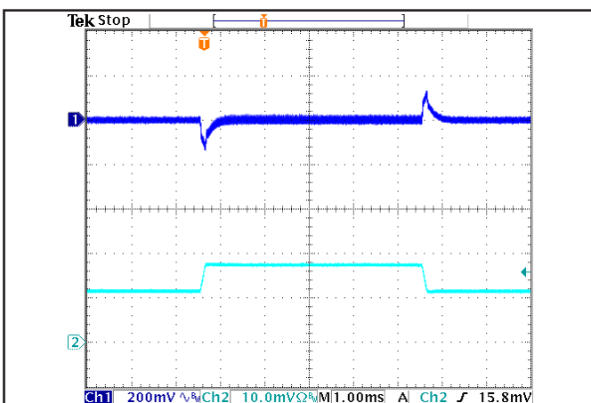
Figure 5: Output voltage response to step-change in load current (50%-75%-50% of Iout(max)); di/dt = 0.1 \text{ A}/\mu\text{s} . Load cap: 15 \mu\text{F} Tantalum + 1 \mu\text{F} Ceramic capacitor. Ch 1: Vout (200 mV/div), Ch 2: Iout (20 A/div).
