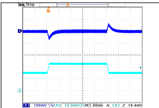
Figure 5: Output voltage response to step-change in load current (50%-75%-50% of I out (max); dI/dt = 0.1 A/μs). Load cap: 15 μF Tantalum + 1 μF Ceramic capacitor. Ch 1: V out (100 mV/div), Ch 2: I out (20 A/div).
