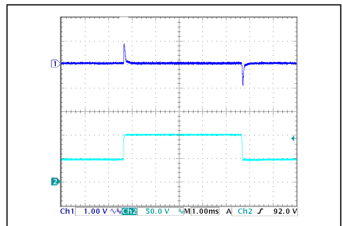
Figure 6: Output voltage response to step-change in input voltage (1000 V/ms). Load cap: 100 µF, electrolytic output capacitance. Ch 1: V out (1 V/div), Ch 2: V in (50 V/div).
