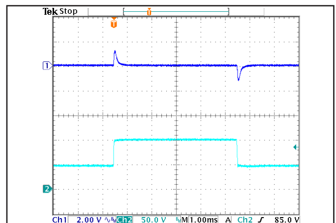
Figure 6: Output voltage response to step-change in input voltage (1000 V/ms). Load cap: 100 μF, electrolytic output capacitance. Ch 1: V out (2 V/div), Ch 2: V in (50 V/div).
