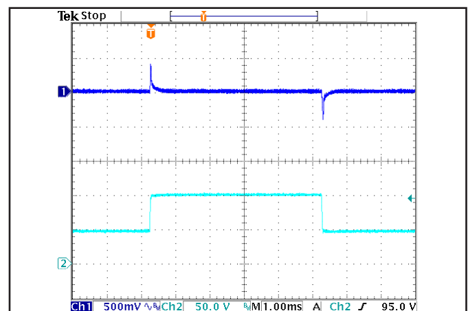
Figure 6: Output voltage response to step-change in input voltage (1000 V/ms). Load cap: 100 \mu\text{F} , electrolytic output capacitance. Ch 1: Vout (500 mV/div), Ch 2: Vin (50 V/div).
