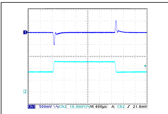
Figure 5: Output voltage response to step-change in load current (50%-75%-50% of I out (max)); dI/dt = 0.1 A/µs. Load cap: 15 µF Tantalum + 1 µF Ceramic capacitor. Ch 1: V out (500 mV/div), Ch 2: I out (5 A/div).
