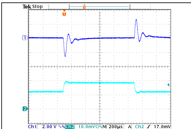
Figure 5: Output voltage response to step-change in load current (50%-75%-50% of I out (max); dl/dt = 0.1 A/us). Load cap: 1 μF ceramic capacitor. Ch 1: V out (2 V/div), Ch 2: I out (2 A/div).
