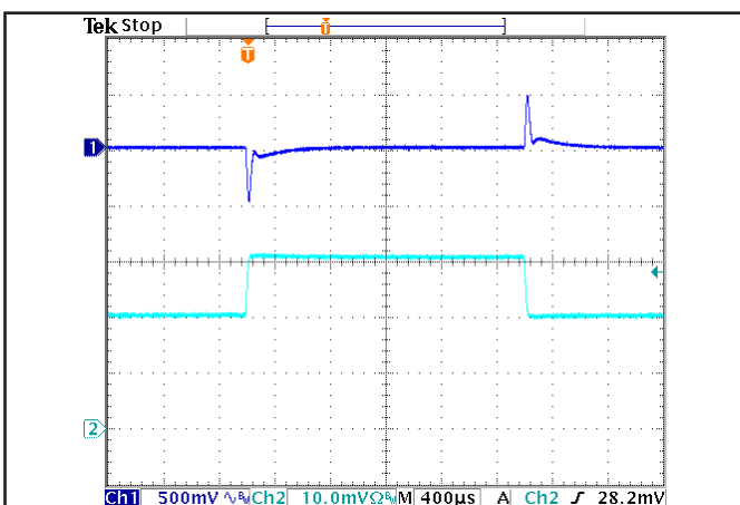
Figure 5: Output voltage response to step-change in load current (50%-75%-50% of I out (max); dI/dt = 0.02 A/μs). Load cap: 15 μF Tantalum + 1 μF Ceramic capacitor. Ch 1: V out (500 mV/div), Ch 2: I out (5 A/div).
