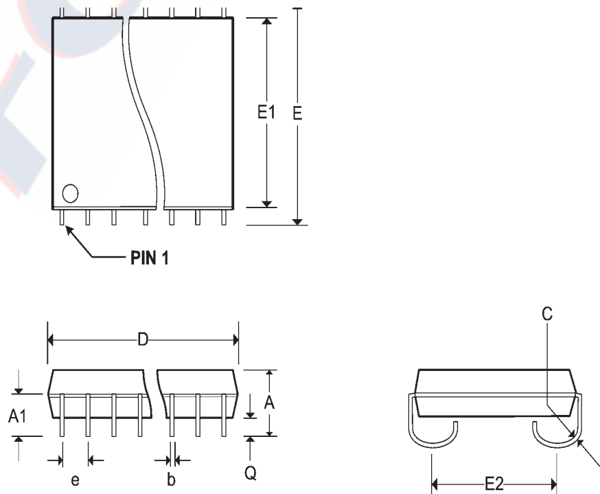
SOJ SMALL OUTLINE IC PACKAGE (400 mil)
