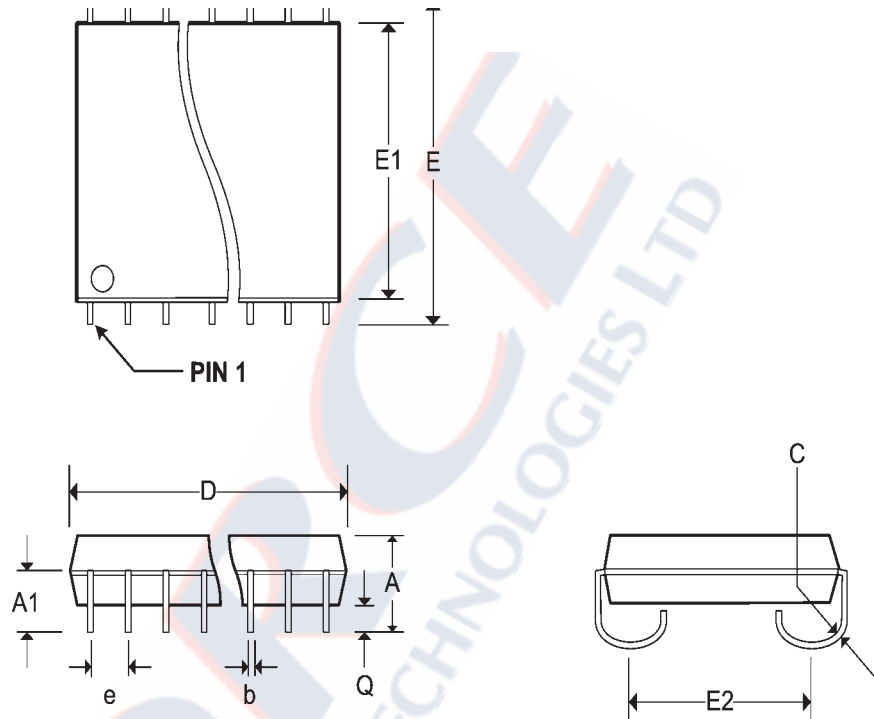
SOJ SMALL OUTLINE IC PACKAGE (300 mil)
