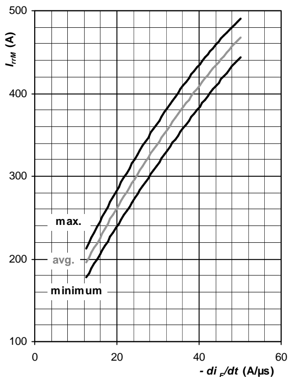
Fig. 11 Reverse recovery maximum current I_{rrm} vs. rate of fall forward current di_F/dt , trapezoid pulse, I_{FM} = 2\ 000\ A , V_R = 100\ V , T_j = T_{jmax}
