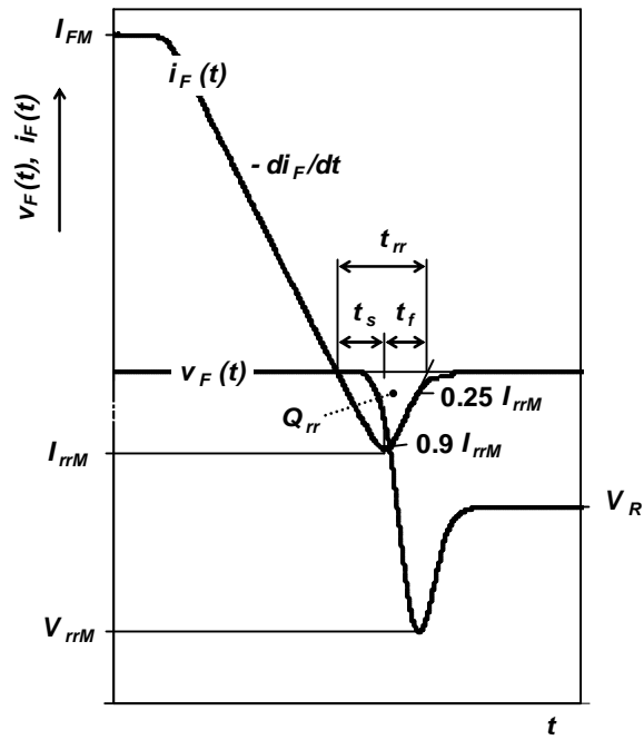
Fig. 13 Typical waveforms and definition of symbols at reverse recovery of a diode
