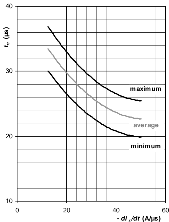
Fig. 12 Reverse recovery time t_{rr} vs. rate of fall forward current di_F/dt , trapezoid pulse, I_{FM} = 2\ 000\ A , V_R = 100\ V , T_j = T_{jmax}
