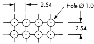
Recommended PC Board Pattern Double Row
