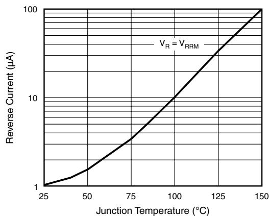
Figure 2. Reverse Current vs. Junction Temperature
