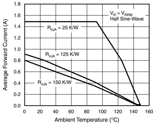
Figure 4. Average Forward Current vs. Ambient Temperature
