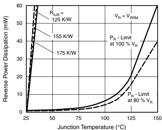
Figure 1. Max. Reverse Power Dissipation vs. Junction Temperature
