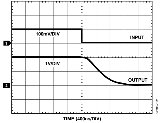
Figure 13. Fall Time
