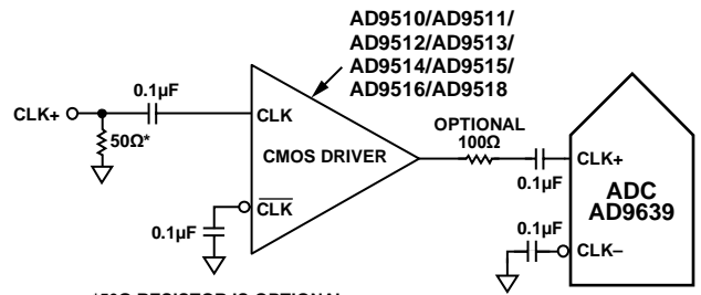
Figure 47. Single-Ended 3.3 V CMOS Sample Clock
