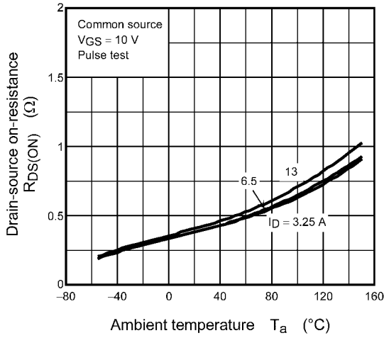
Fig. 8.7 R DS(ON) - T a
