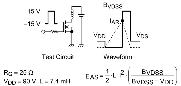
Fig. 8.16 Test Circuit/Waveform
