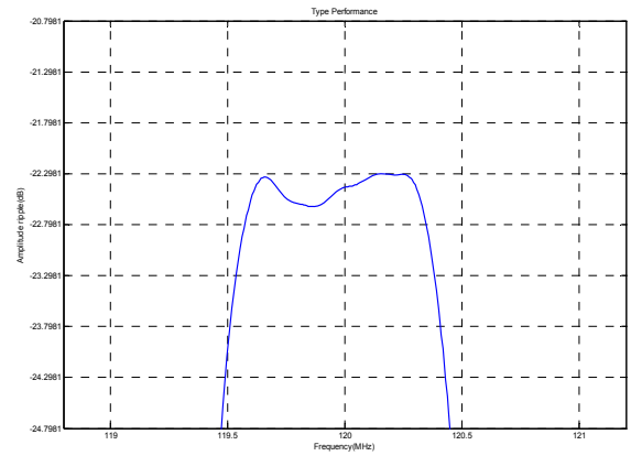
Passband Respond
