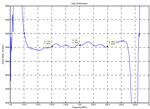
Group Delay Variation(f0±0.4MHz)
