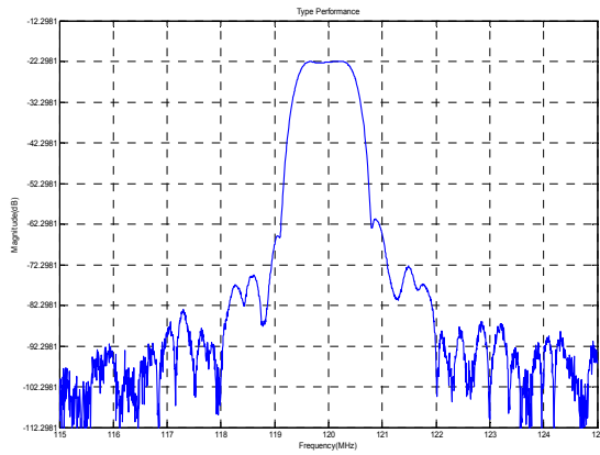
Frequency Respond
