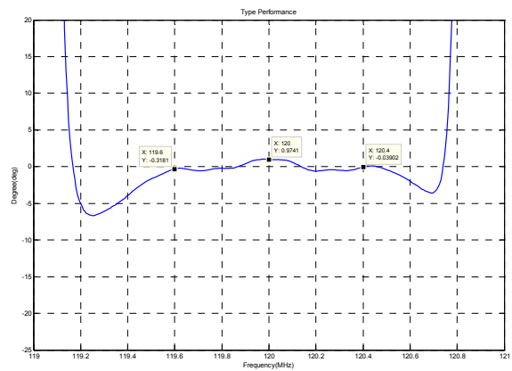
Phase Linearity(f0±0.4MHz)
