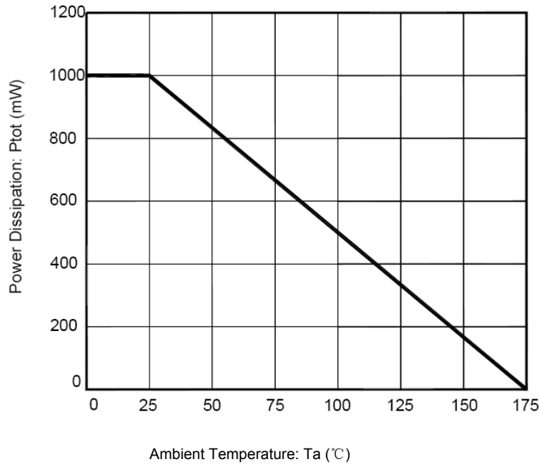
Power Dissipation vs Ambient Temperature
