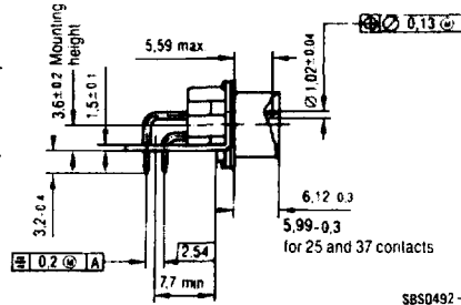
Female connector
