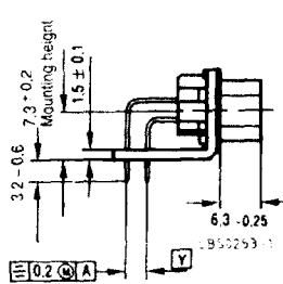
Female connector
