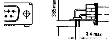
Version with mounting clips
