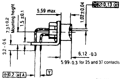
Pin connector
