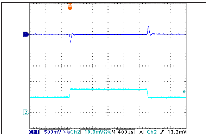
Figure 5: Output voltage response in the SM version to step-change in load current (50%-75%-50% of I out (max); dI/dt = 0.1 A/µs). Load cap: 100 µF electrolytic cap and 1 µF ceramic cap. Ch 1: V out (500 mV/div), Ch 2: I out (5 A/div).
