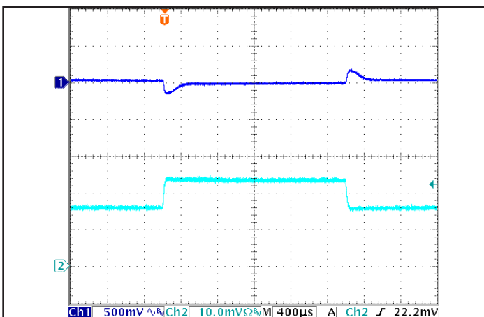
Figure 5: Output voltage response in the SM version to step-change in load current (50%-75%-50% of I out (max); dI/dt = 0.1 A/μs). Load cap: 100 μF electrolytic cap and 1 μF ceramic cap. Ch 1: V out (500 mV/div), Ch 2: I out (1 A/div).
