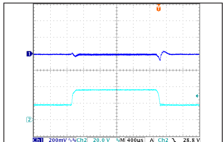
Figure 6: Output voltage response in the SM version to step-change in input voltage (250 V/ms). Load cap: 100 μF, electrolytic output capacitance. Ch 1: V out (200 mV/div), Ch 2: V in (20 V/div).
