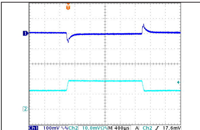
Figure 5: Output voltage response in the SM version to step-change in load current (50%-75%-50% of Iout(max); dI/dt = 0.1 A/μs). Load cap: 100 μF electrolytic cap and 1 μF ceramic cap. Ch 1: Vout (100 mV/div), Ch 2: Iout (10 A/div).
