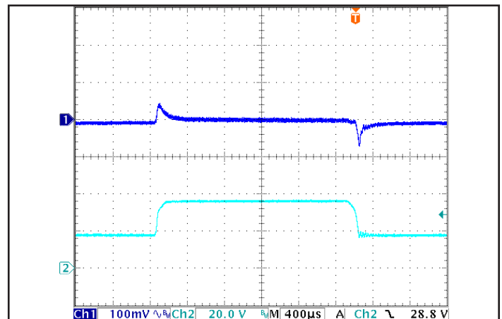
Figure 6: Output voltage response in the SM version to step-change in input voltage (250 V/ms). Load cap: 100 µF, electrolytic output capacitance. Ch 1: V out (100 mV/div), Ch 2: V in (20 V/div).
