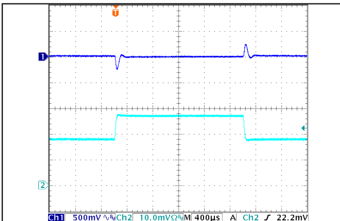
Figure 5: Output voltage response in the SM version to step-change in load current (50%-75%-50% of Iout(max); dI/dt = 0.1 A/μs). Load cap: 100 μF electrolytic cap and 1 μF ceramic cap. Ch 1: Vout (500 mV/div), Ch 2: Iout (2 A/div).
