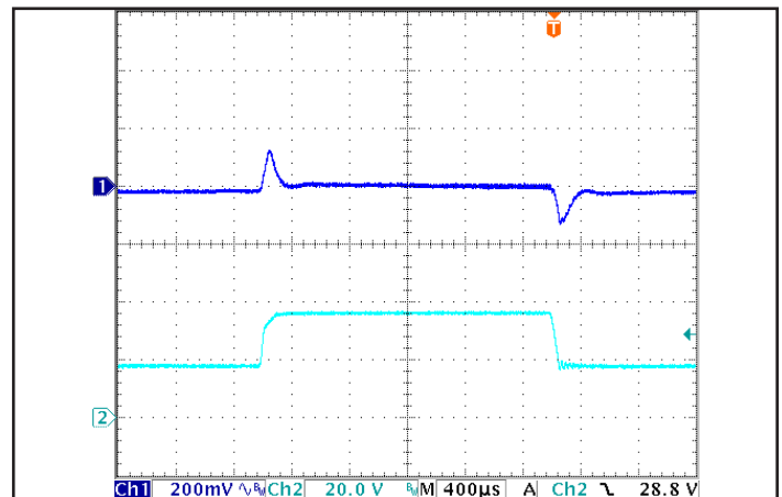
Figure 6: Output voltage response in the SM version to step-change in input voltage (250 V/ms). Load cap: 100 µF, electrolytic output capacitance. Ch 1: V out (200 mV/div), Ch 2: V in (20 V/div).
