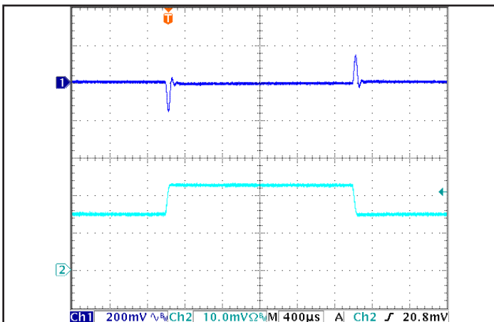
Figure 5: Output voltage response in the SM version to step-change in load current (50%-75%-50% of Iout(max)); dI/dt = 0.1 A/μs. Load cap: 100 μF electrolytic cap and 1 μF ceramic cap. Ch 1: Vout (200 mV/div), Ch 2: Iout (5 A/div).
