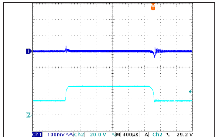
Figure 6: Output voltage response in the SM version to step-change in input voltage (250 V/ms). Load cap: 100 μF, electrolytic output capacitance. Ch 1: Vout (100 mV/div), Ch 2: Vin (20 V/div).
