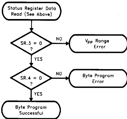
Figure 6. Automated Byte Programming Flowchart
