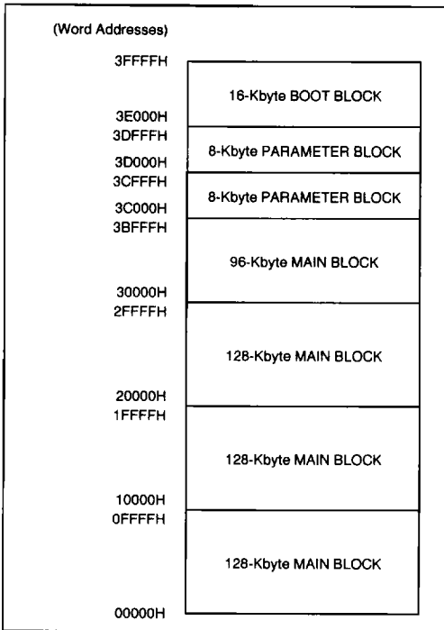
Figure 5. A28F400BX-T Memory Map
