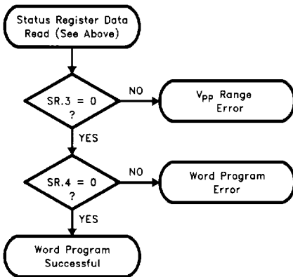
Figure 7. Automated Word Programming Flowchart
