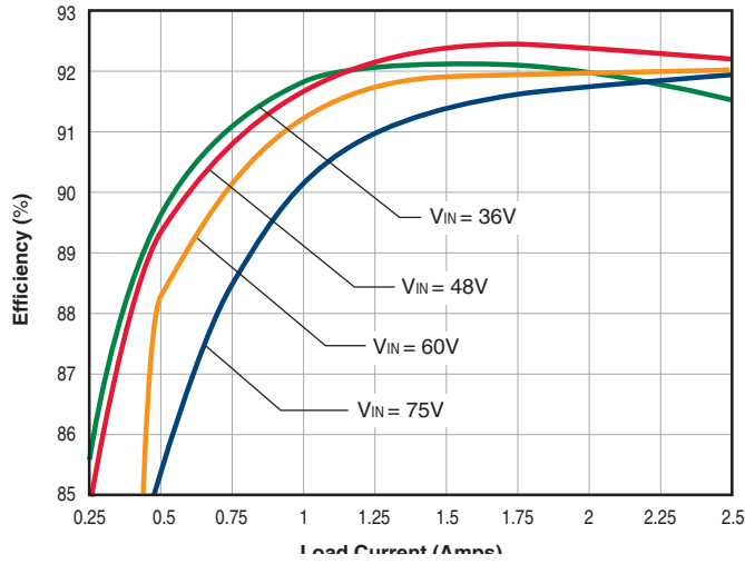
UVQ-48/2.5-D48N Efficiency vs. Line Voltage and Load Current @ 25°C
