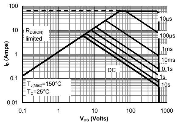
Figure 12: Maximum Forward Biased Safe Operating Area for AOWF15S60 (Note F)
