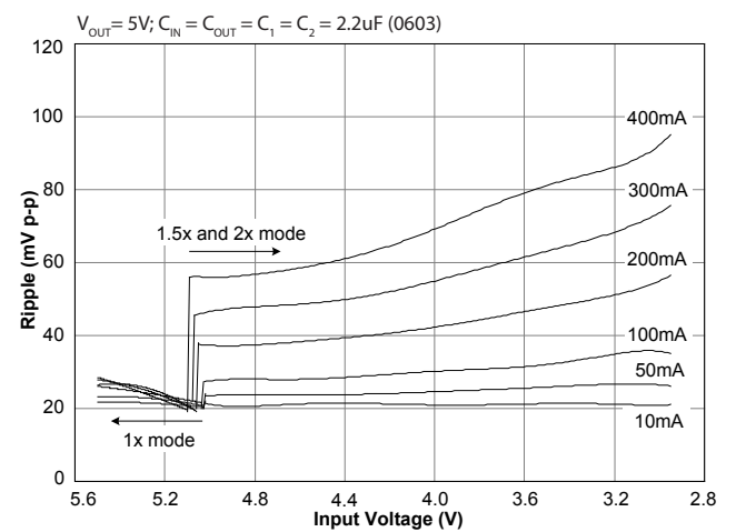
Output Ripple
