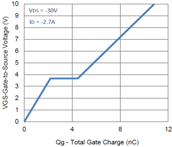
7. Gate Charge
