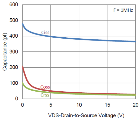
6. Capacitance
