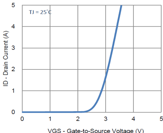
2. Transfer Characteristics
