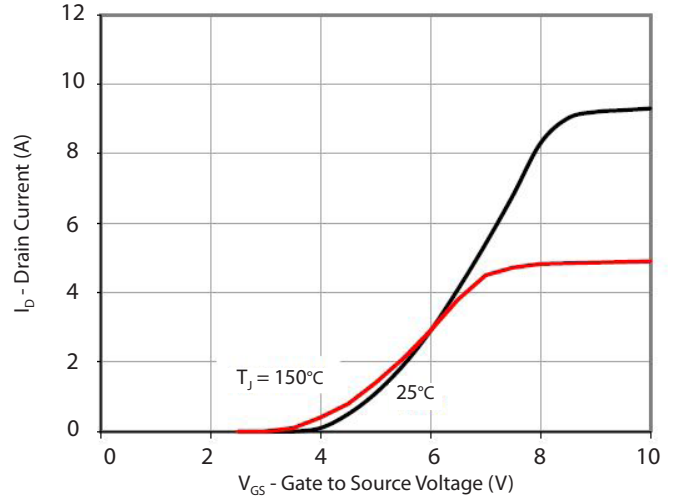
Transfer Characteristics
