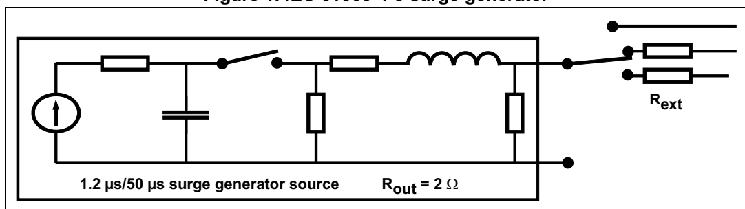
Figure 1. IEC 61000-4-5 surge generator
