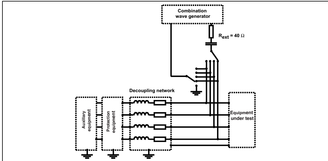
Figure 6. IEC 61000-4-5 multi-line test set-up
