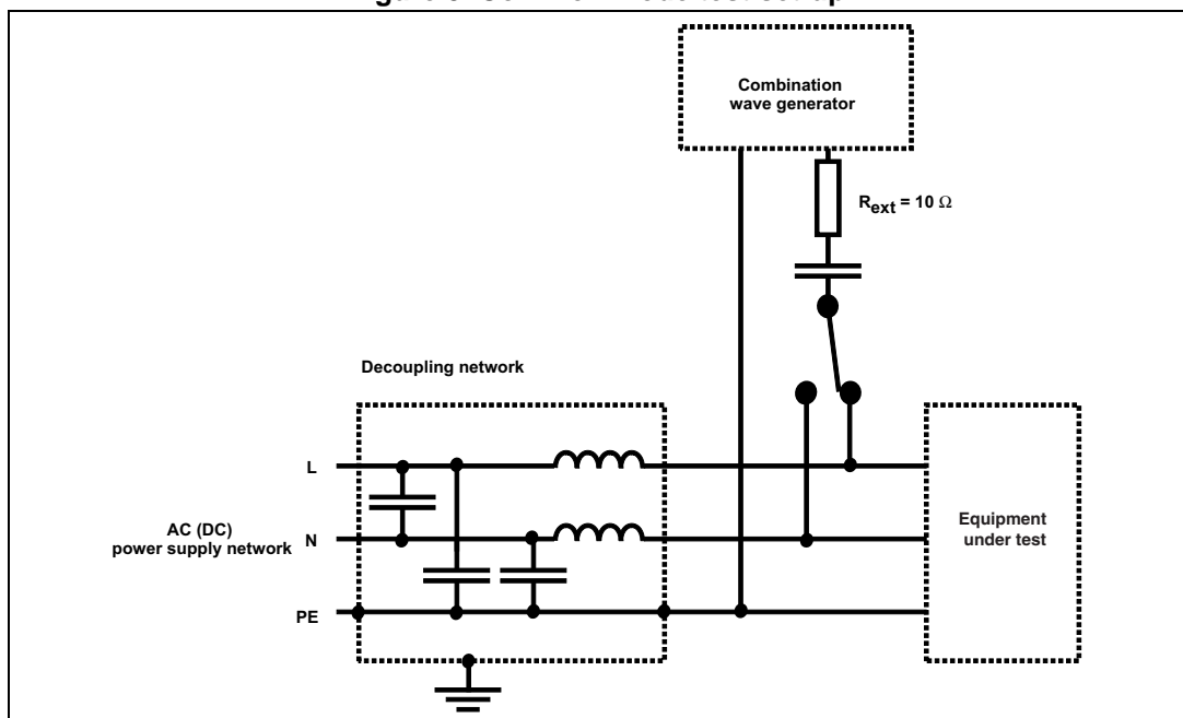
Figure 5. Common mode test set-up
