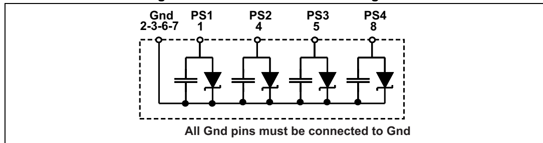
Figure 8. PEP01-5841 functional diagram
