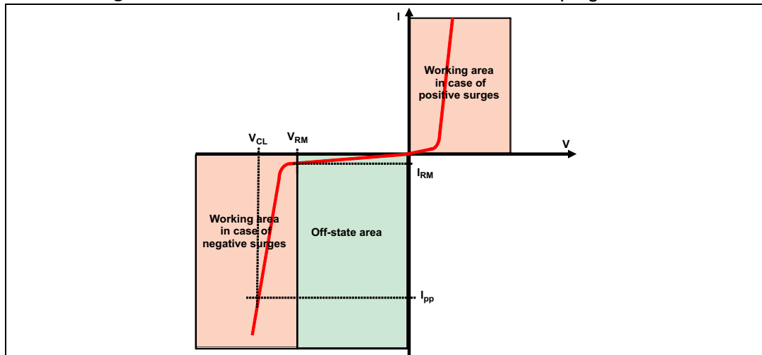
Figure 7. I/V characteristics of a unidirectional clamping devices
