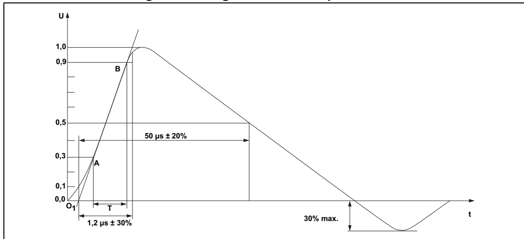
Figure 2. Voltage waveform in open circuit
