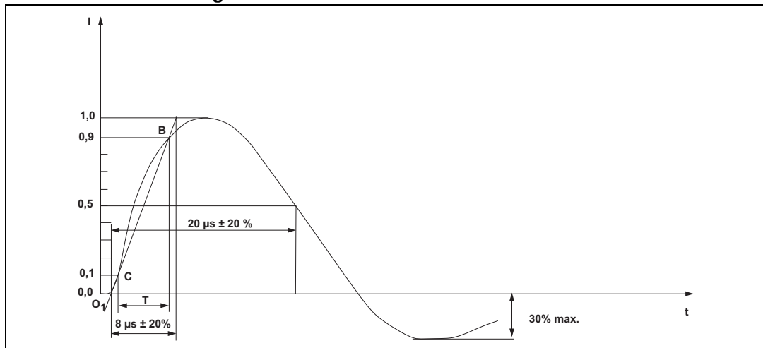
Figure 3. Current waveform in short circuit
