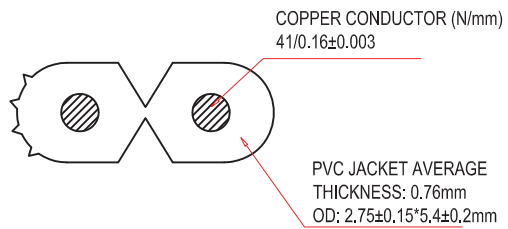
Wire cross section
