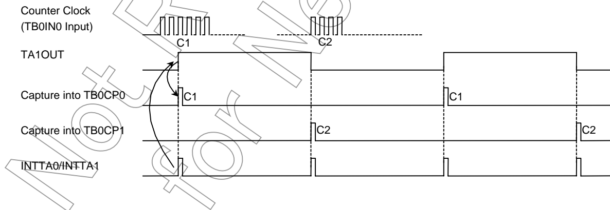
Figure 12.12 Frequency Measurement
