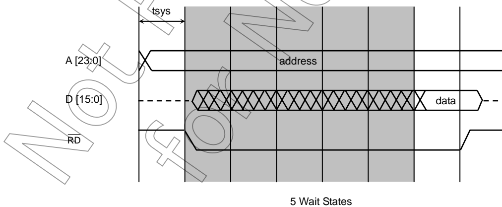
Figure 8.4 Read Cycle Timing (with Automatically Inserted Five Wait States)
