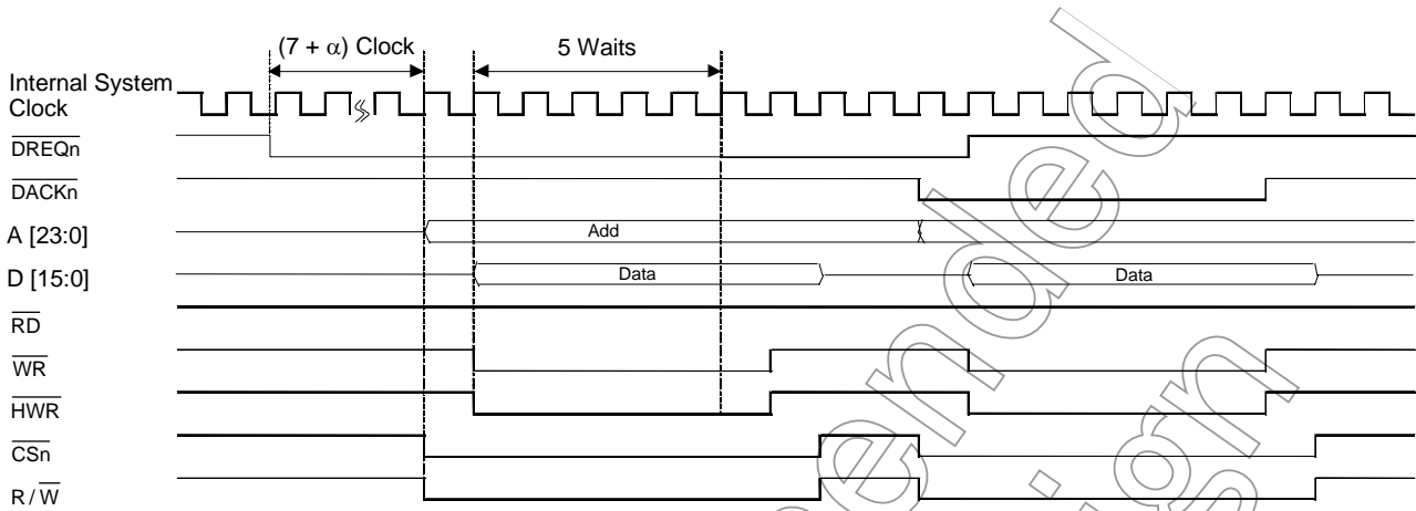
Figure 10.21 Level Mode (Transfer from the On-chip RAM to an External Memory)
