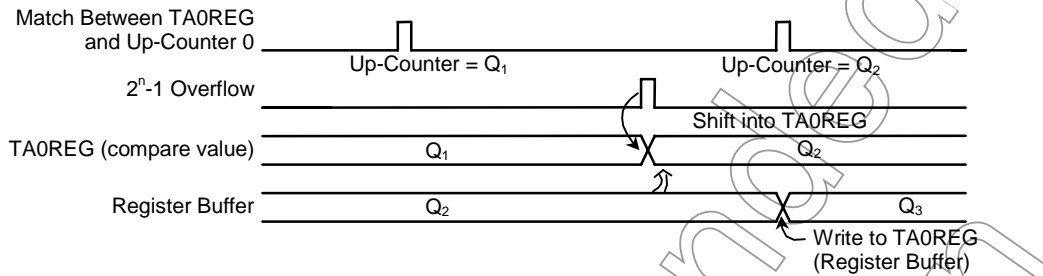
Figure 11.11 Register Buffer Operation
