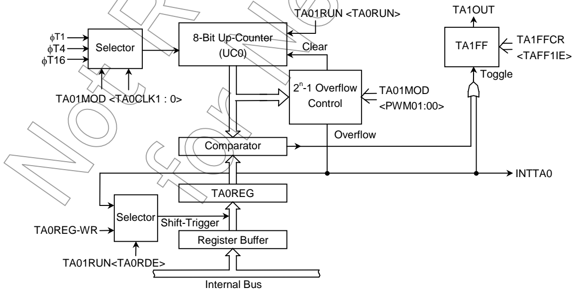
Figure 11.10 Functional Diagram of 8-Bit PWM Generation Mode
