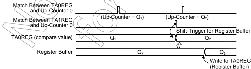
Figure 11.8 Register Buffer Operation
