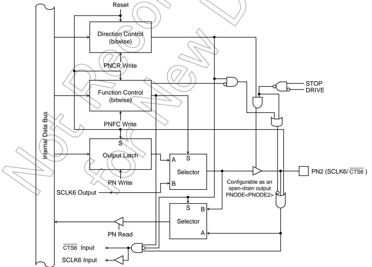
Figure 7.67 Port N (PN2)
