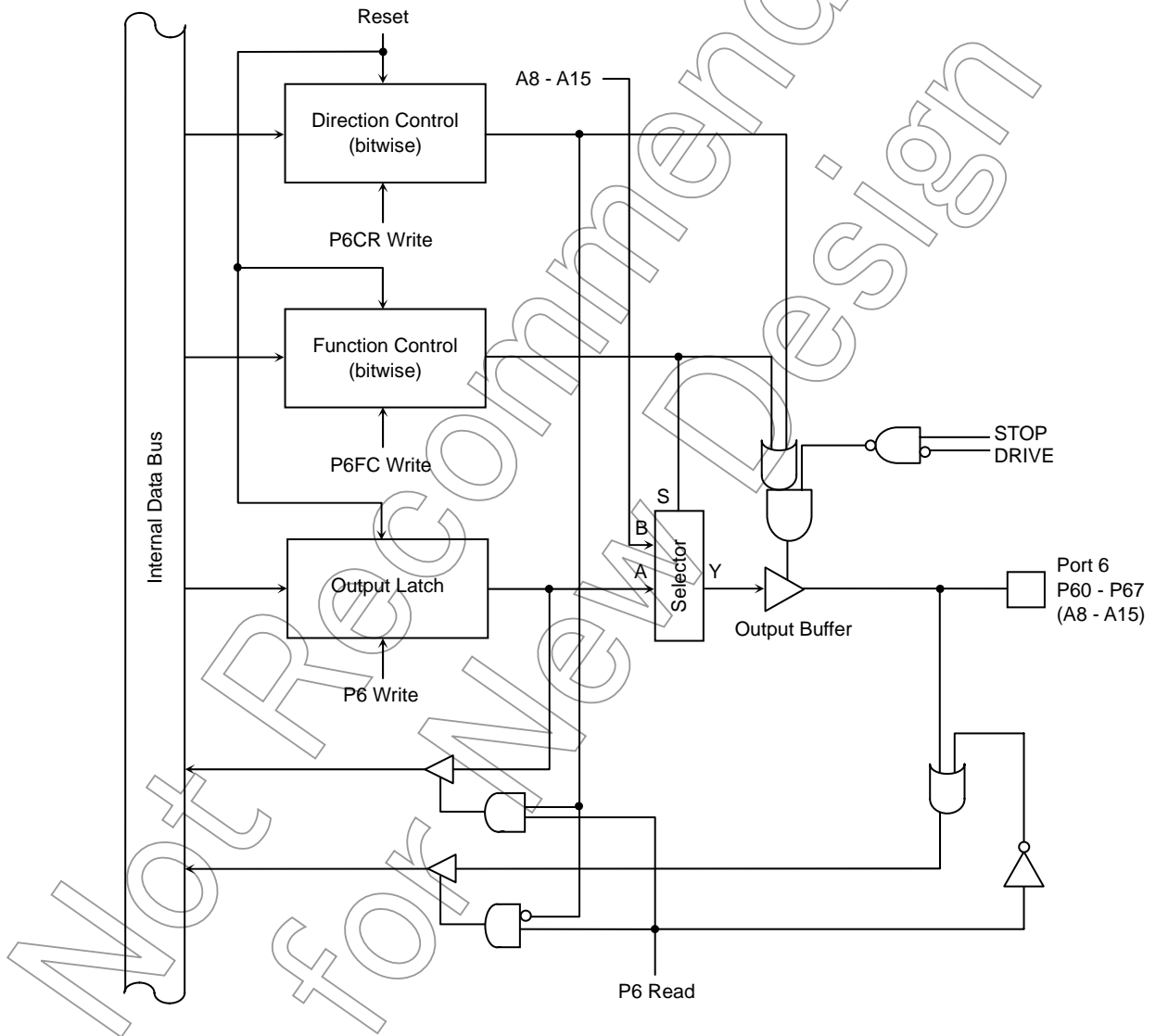
Figure 7.17 Port 6 (P60 - P67)
