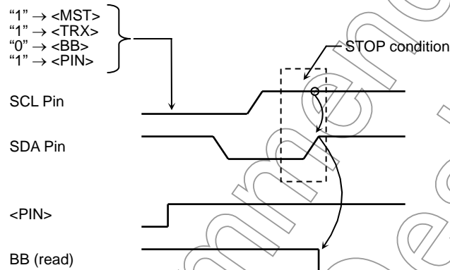
Figure 15.18 Generating a STOP Condition
