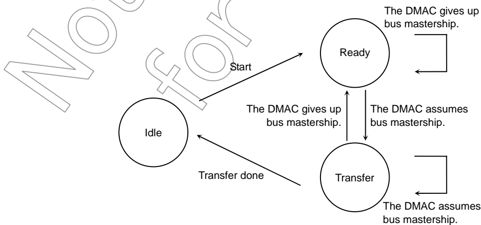
Figure 10.12 DMA Channel State Transitions
