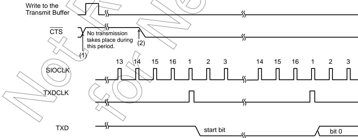
Figure 14.4 Handshaking Signals
