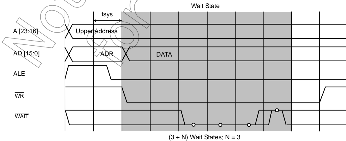
Figure 8.29 Write Cycle Timing (with (3 + N) Wait States; N = 3)
