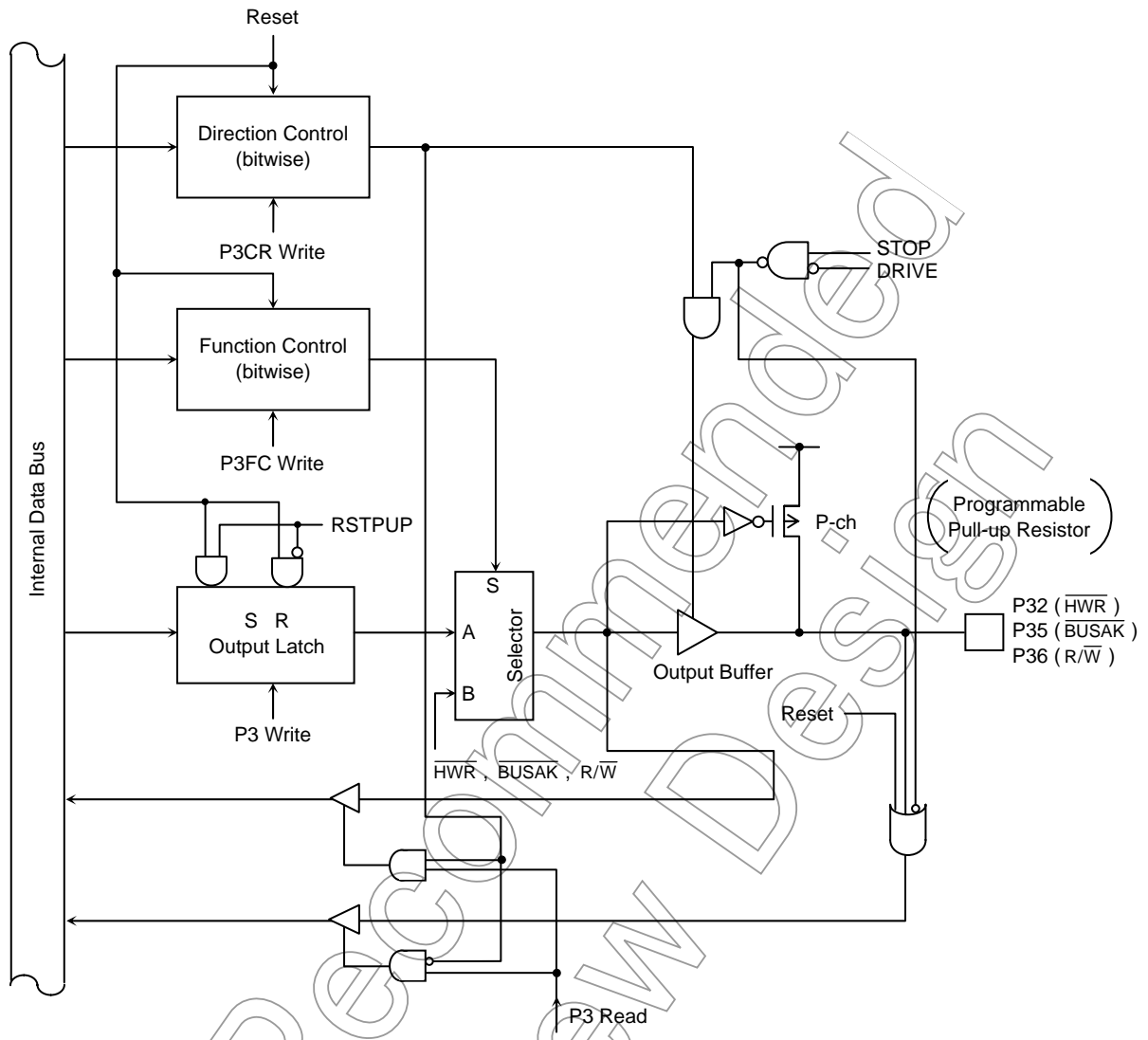
Figure 7.8 Port 3 (P32, P35, P36)
