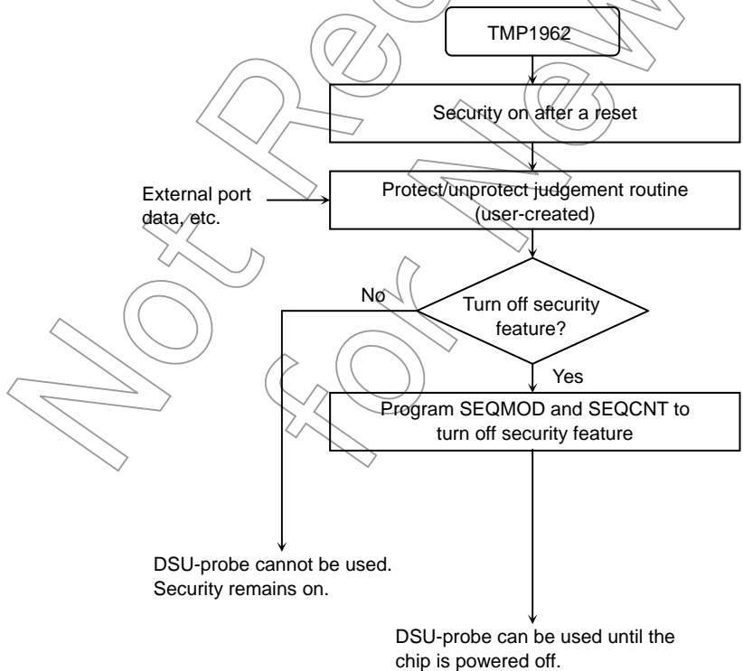
Figure 20.1 Using the Security Feature
