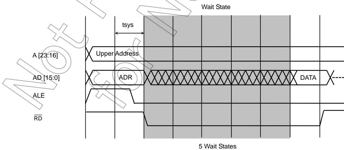
Figure 8.21 Read Cycle Timing (with Five Wait States)
