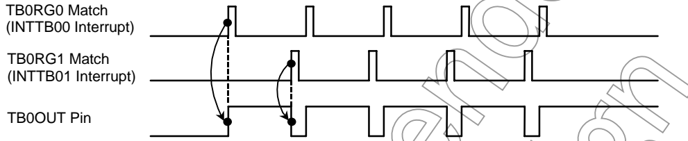
Figure 12.7 PPG Output Waveform
