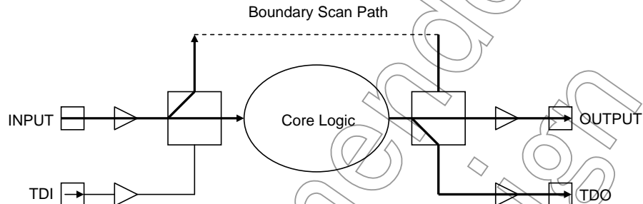
Figure 21.9 Test Data Flow While SAMPLE is Selected
