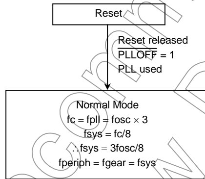
Figure 5.2 Default Clock Frequencies in Normal Mode
