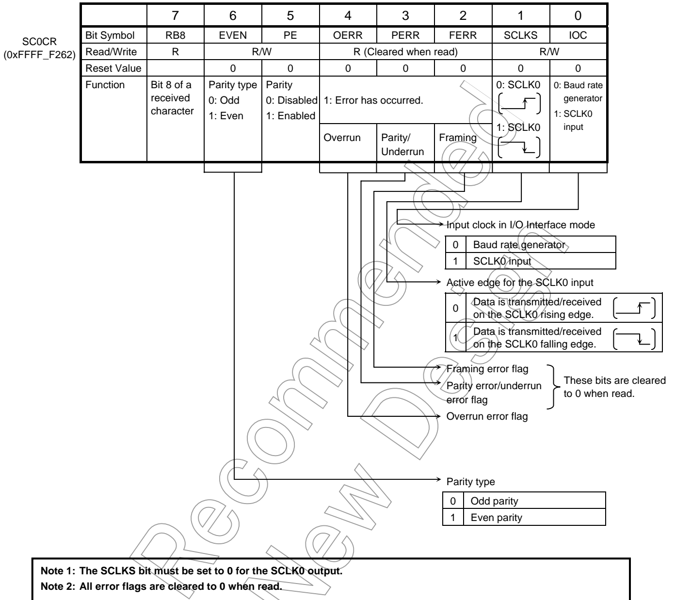
Figure 14.9. Serial Control Register (SC0CR, for SIO0)
