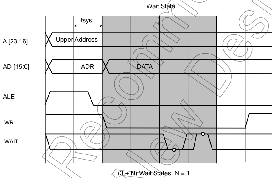
Figure 8.28 Write Cycle Timing (with (3 + N) Wait States; N = 1)
