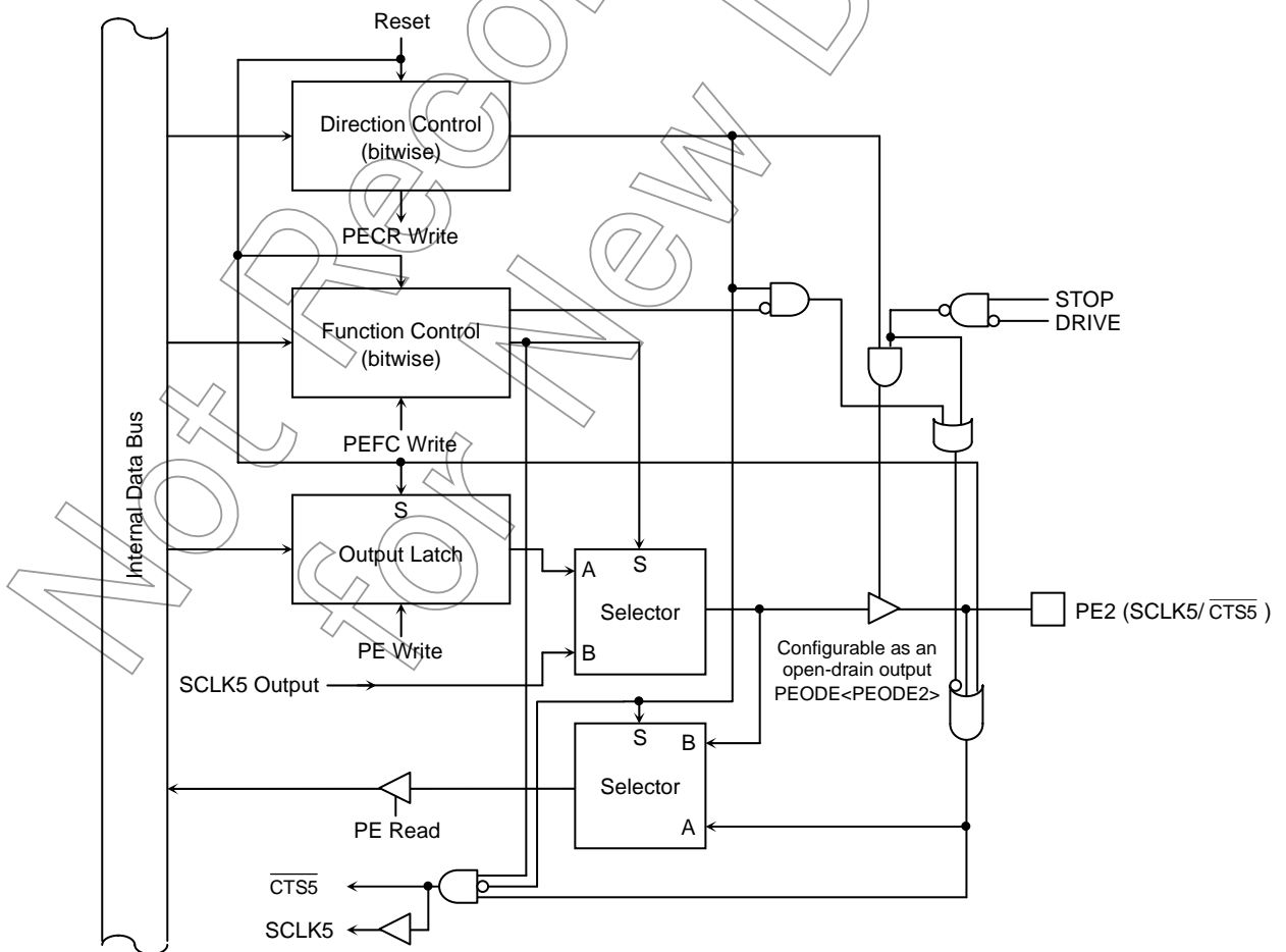
Figure 7.38 Port E (PE2)
