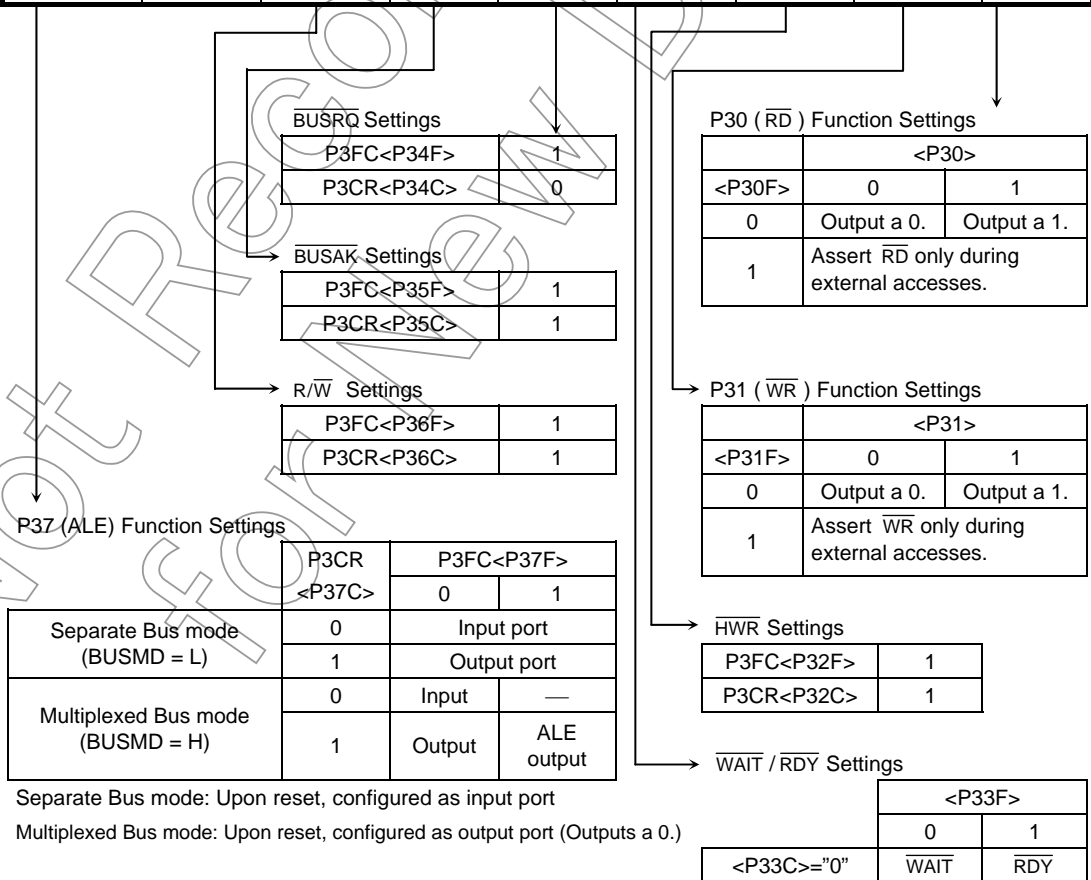
Figure 7.11 Port 3 Registers
