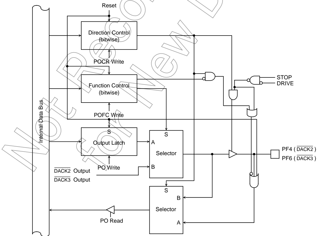
Figure 7.45 Port F (PF4, PF6)
