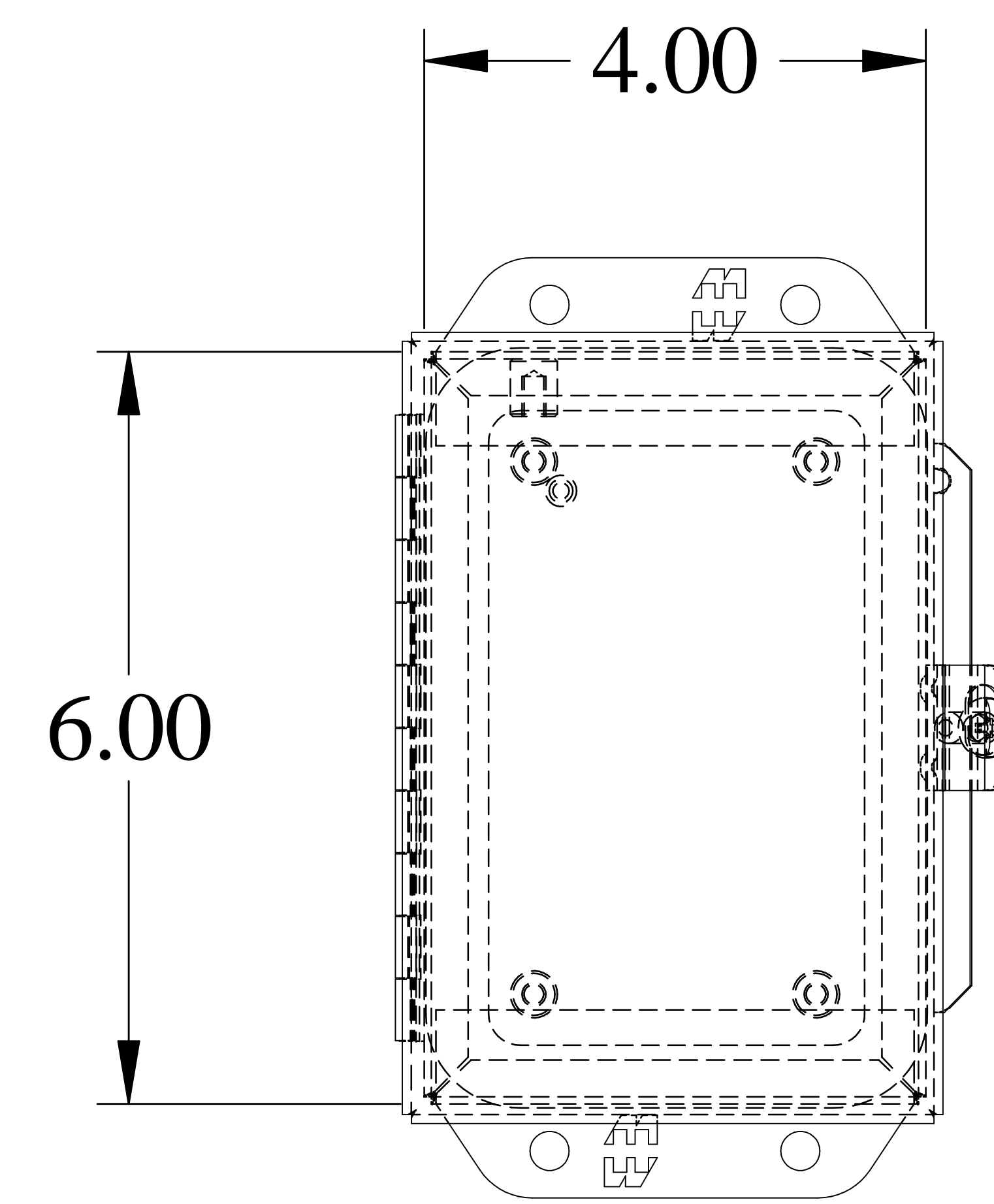
FRONT VIEW
