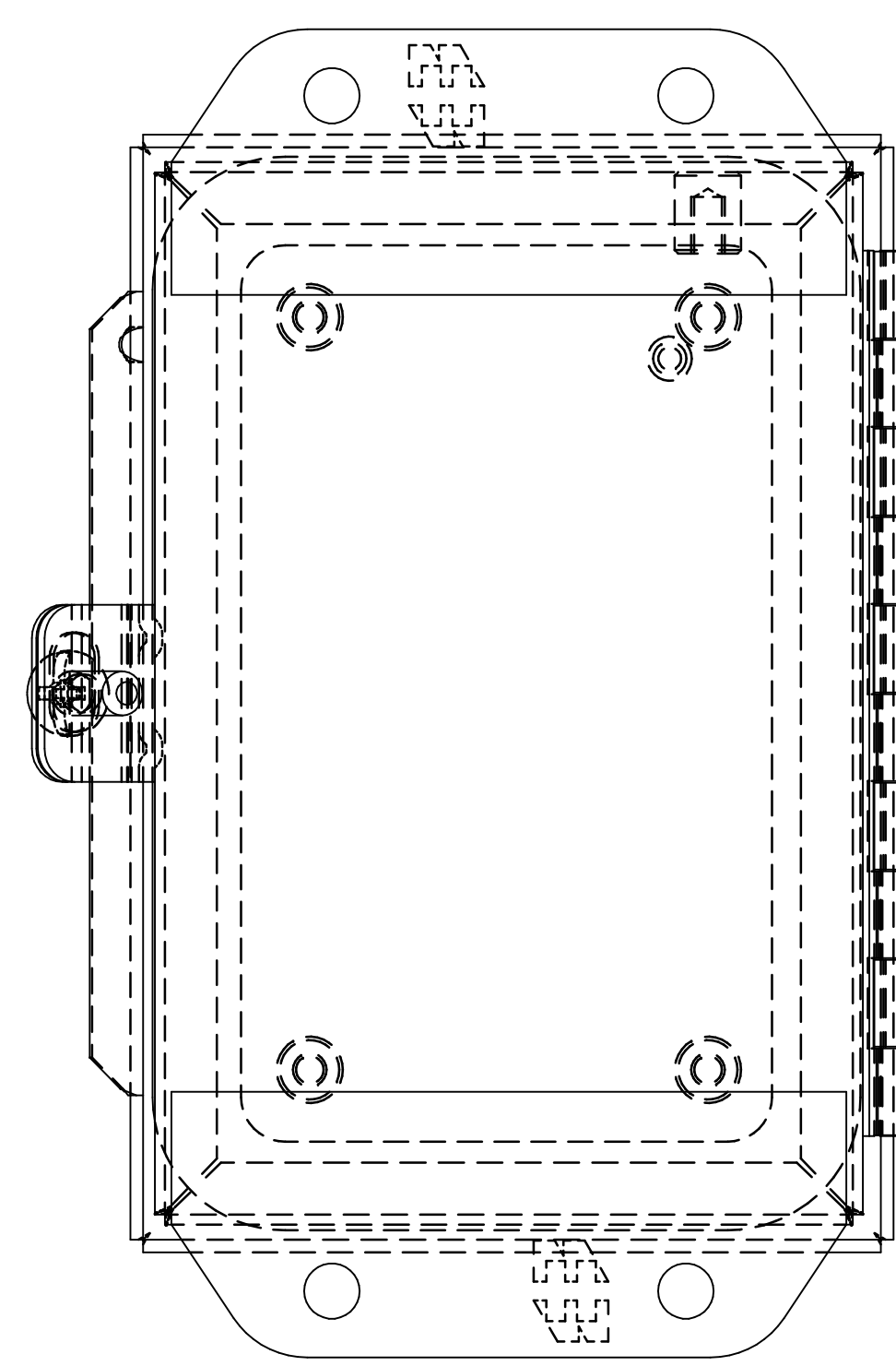
BACK VIEW
