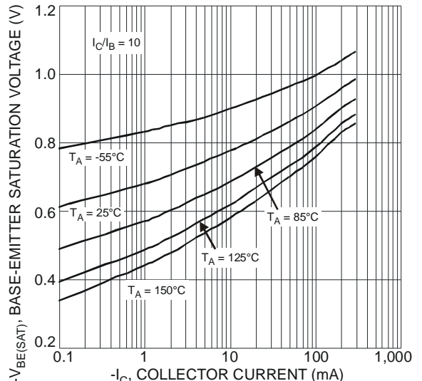
Fig. 15 Typical Base-Emitter Saturation Voltage vs. Collector Current
