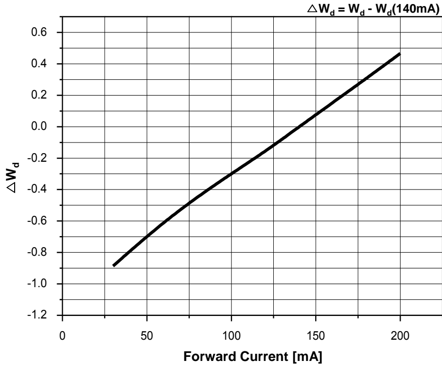
Fig 5. Forward Current vs. W_d Shift , T_a = 25^\circ\text{C}
