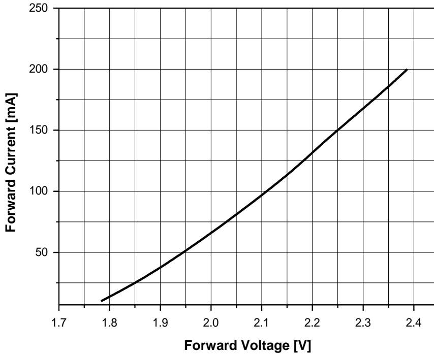
Fig 3. Forward Voltage vs. Forward Current , T_a = 25^\circ\text{C}
