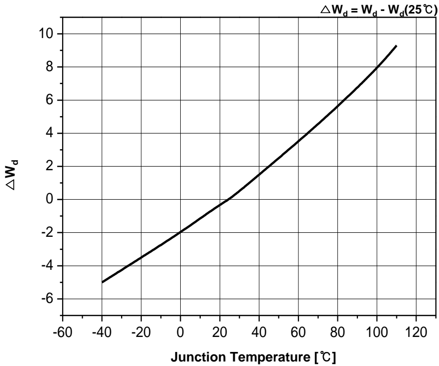
Fig 8. Dominant wavelength shift vs. Junction Temperature, I_F = 140\text{mA}
