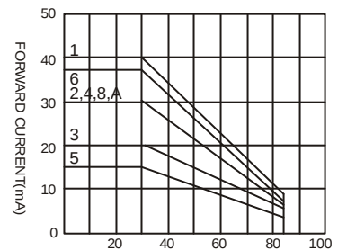
FORWARD CURRENT VS. AMBIENT TEMPERATURE
