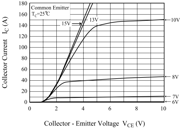
Fig 1. Saturation Voltage Characteristics
