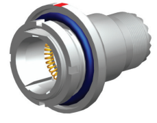
2M804-004-07 Rear Mount Jam Nut with Rear Accessory Threads
