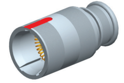
2M804-003-01 In-Line with Integral Backshell
